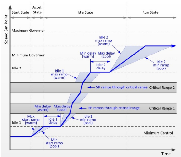
Figure 5. Automatic Start Sequence
