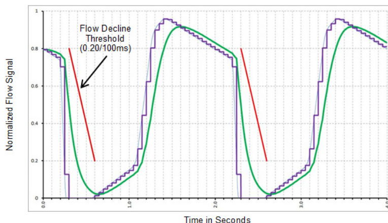
Figure 5 – Surge Digital Signal Profile (with 20 Samples per second) and 100ms Time Constant
