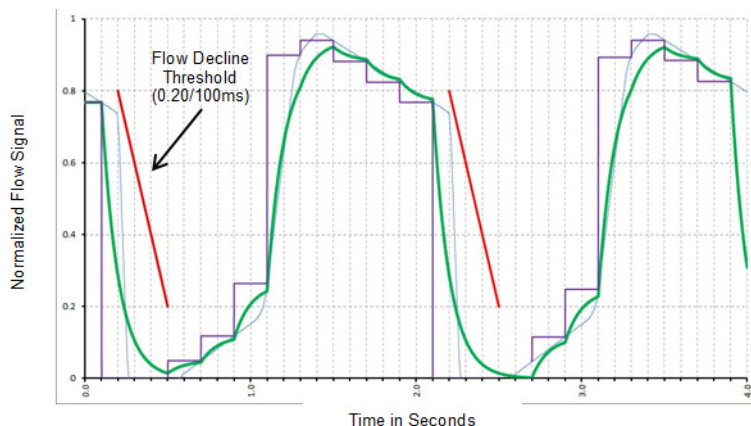
Figure 3 – Surge Digital Signal Profile (with 5 Samples per second) and 100ms Time Constant
