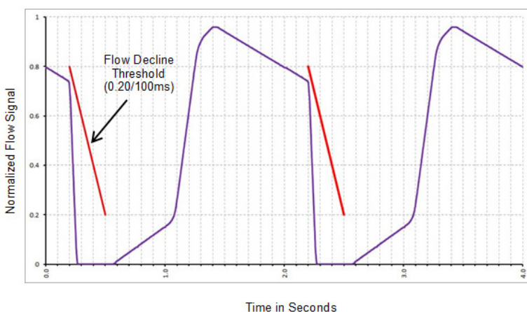
Figure 1 – Surge Analog Flow Signal Profile
