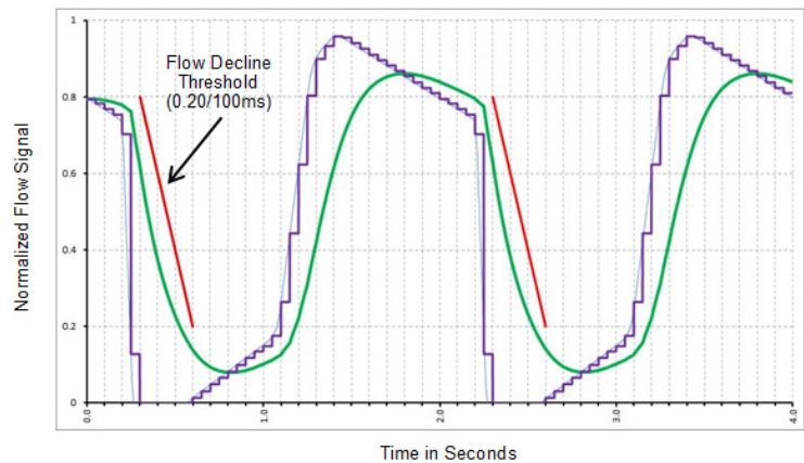
Figure 6 – Surge Digital Signal Profile (with 20 Samples per second) and 200 ms Time Constant
