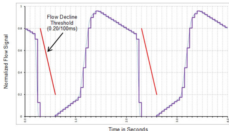
Figure 4 – Surge Digital Signal Profile (with 20 Samples per second) and No Time Constant
