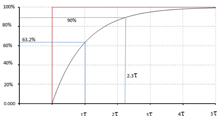
Figure 7 – Difference Between 1st Order Lag Time Constant and API 670 Response Time
