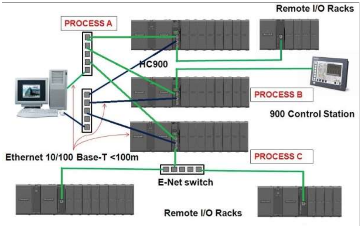
Figure 5 - MULTIPLE PROCESS/MULTIPLE RACKS – RED NETWORKS (STAR TOPOLOGY)
