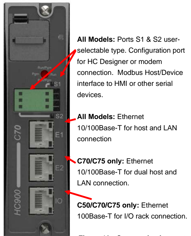
Figure 10 - Communication ports
